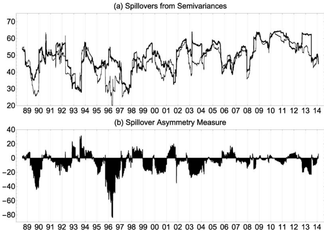
Figure 3: Total Spillover Plot using (a) R^{S+} (thin) and R^{S-} (bold) Semivariance for Crude Oil, Heating Oil, and Gasoline over the Sample Period Extending from September 1, 1987 through February 12, 2014. (b) Spillover Asymmetry Measure (SAM)
