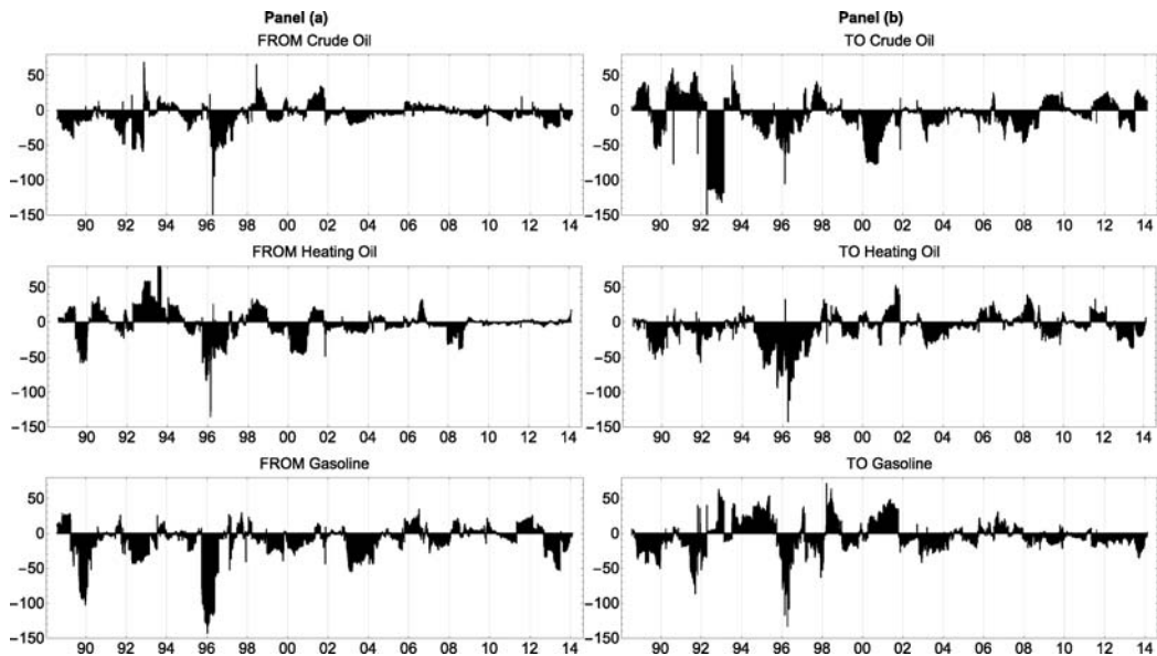
Figure 6: Asymmetric Directional Spillover Plots. Panel (a): Direction FROM ( SAM_{i \rightarrow} ). Panel (b): Direction TO ( SAM_{i \leftarrow} ).
